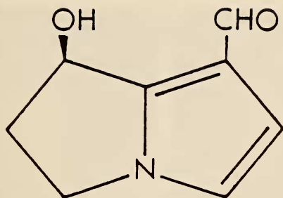
FIG. 1. R-(-)-hydroxydanaidal.
